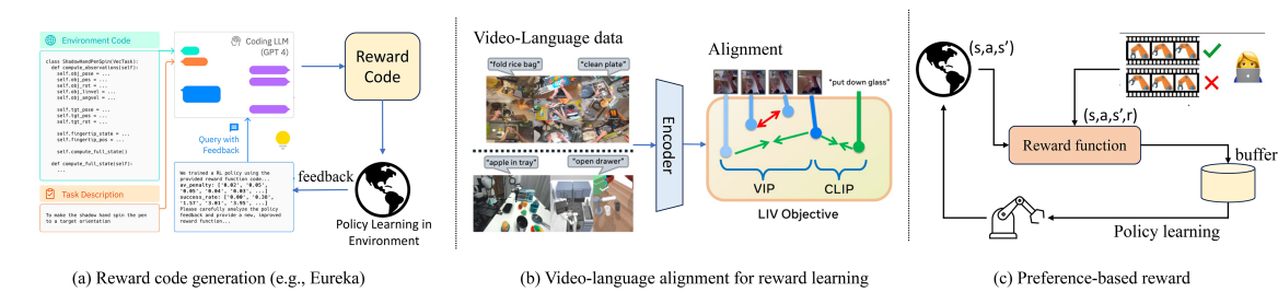
图 15 (网络版彩图) 基于大模型的奖励生成框架对比 Figure 15 (Color online) Comparison of reward generation methods based on foundation models
